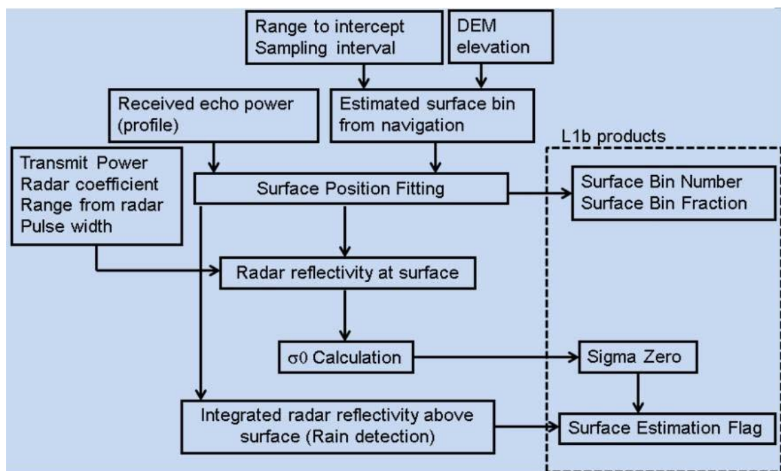
Figure 4.7 Processing flow for surface echo range
