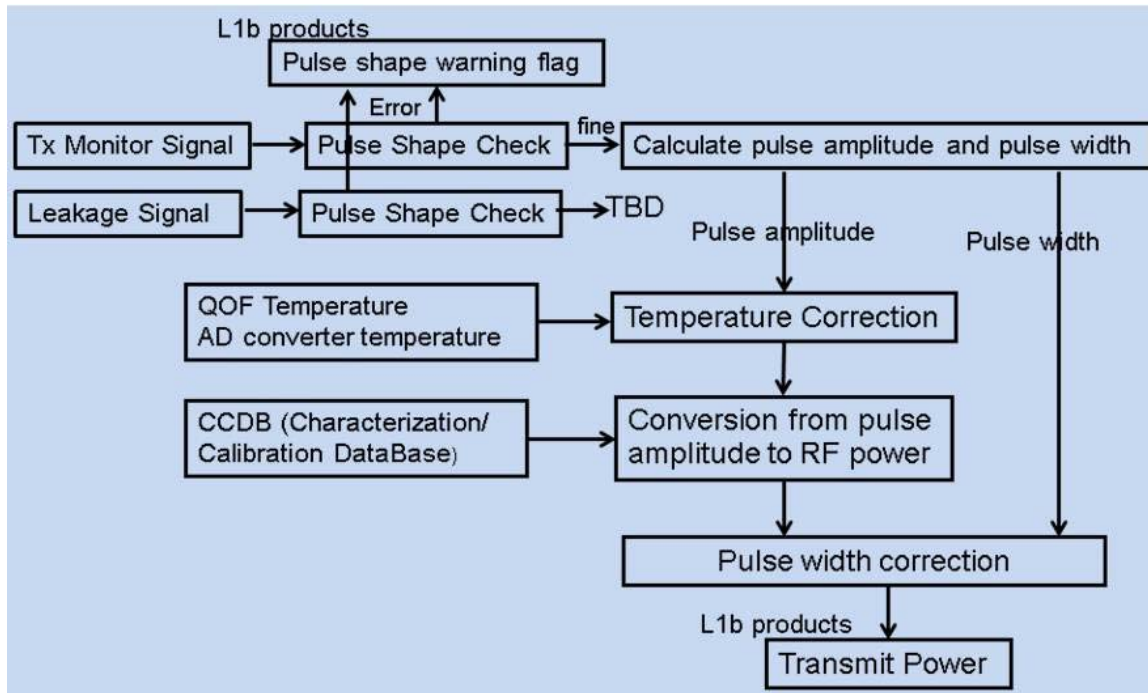
Figure 4.6 Transmit power calculation flow
