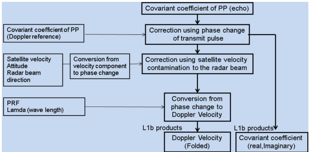
Figure 4.4 Doppler processing in L1b.
