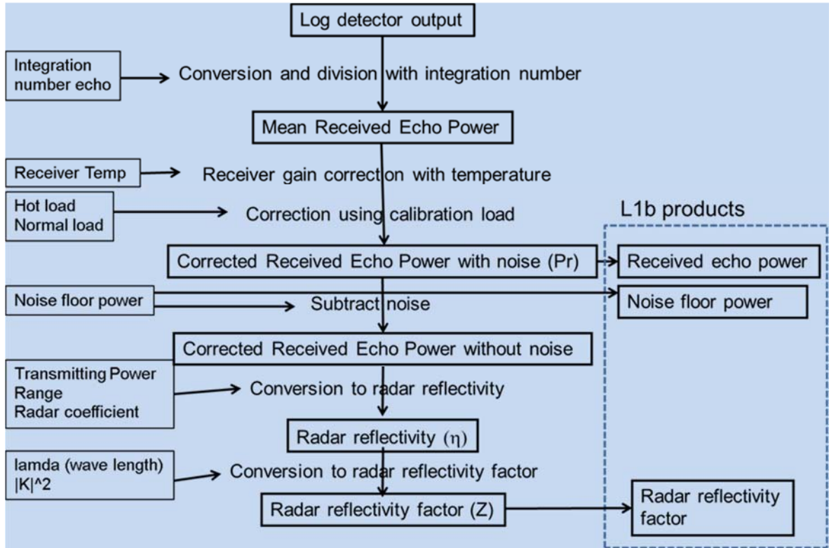
Figure 4.1 Processing for received echo power and radar reflectivity factor
