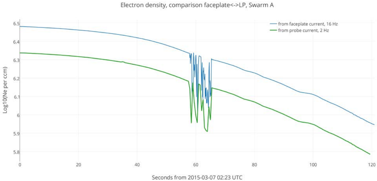
Figure 1: Comparison of densities from the faceplate and probe currents for a short period of 2 minutes.
