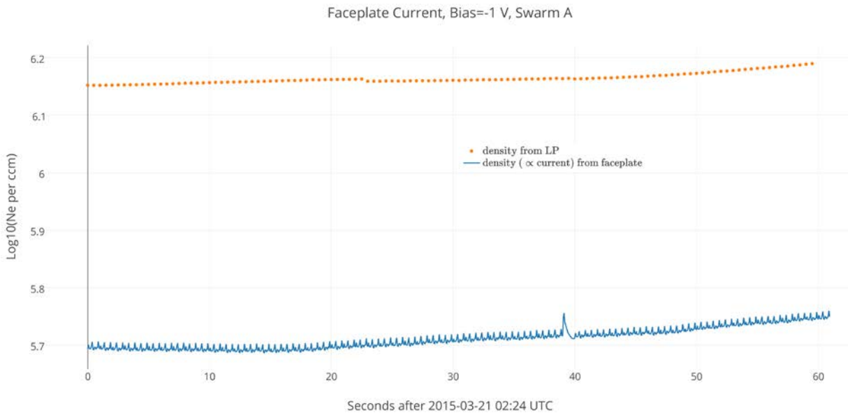
Figure 2: Comparison of densities from the faceplate and probe currents when the faceplate bias is -1 V. A sweep occurs just before second 40.
